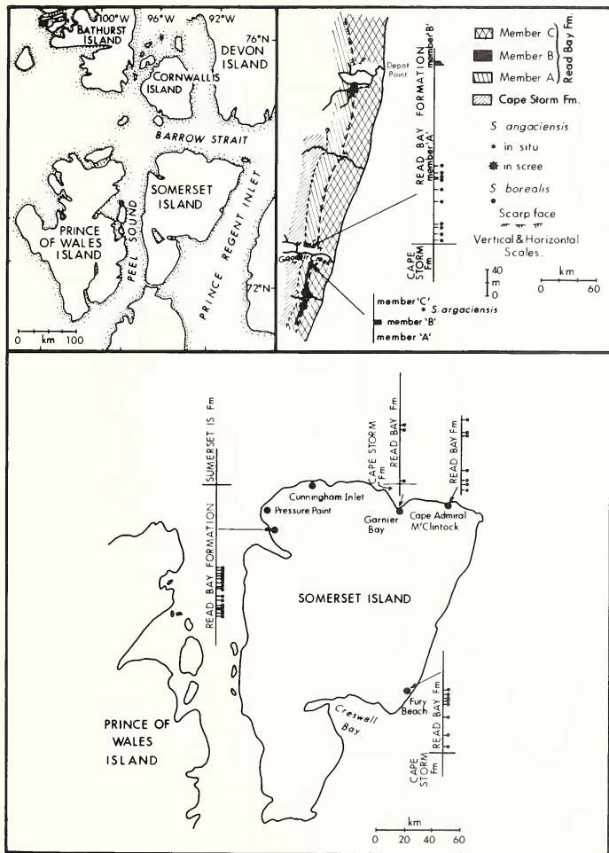
TEXT-FIG. 5. Geographic and stratigraphic locations of Stegerhynchus borealis and S. angaciensis in the Read Bay Formation of Somerset, Prince of Wales, and Cornwallis Islands. S. borealis is relatively common, especially in the lower part of the formation whereas S. angaciensis is relatively rare, occurring only in the basal part of Member C on eastern Cornwallis Island.
